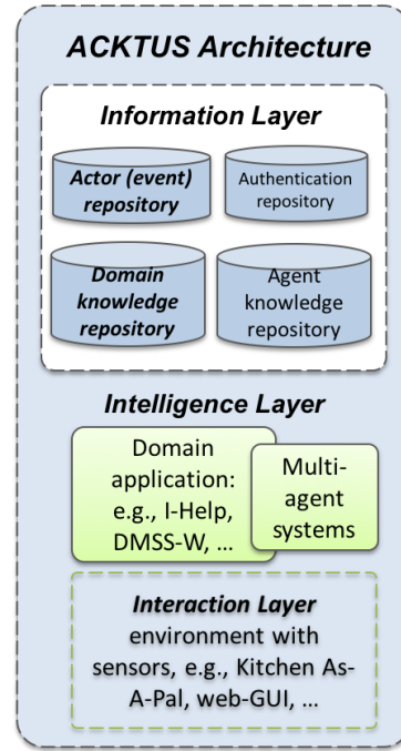
Figure 4: An overview of the ACKTUS architecture that implements the model.
