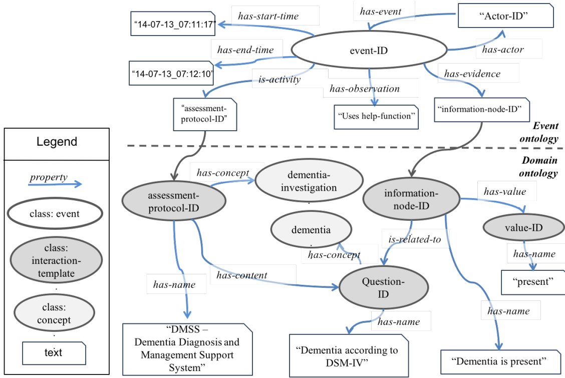
Figure 2: Example from the dementia domain of protocol-based activity .
